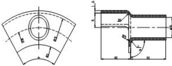
直筒引线反角环片 Snout Sectors of Angle Caps
