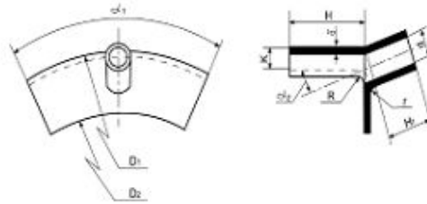
斜筒引线反角环片 Inclined Snout of Angle Caps
