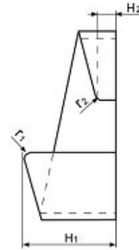
铁轭绝缘端圈 Collars with Spacers
